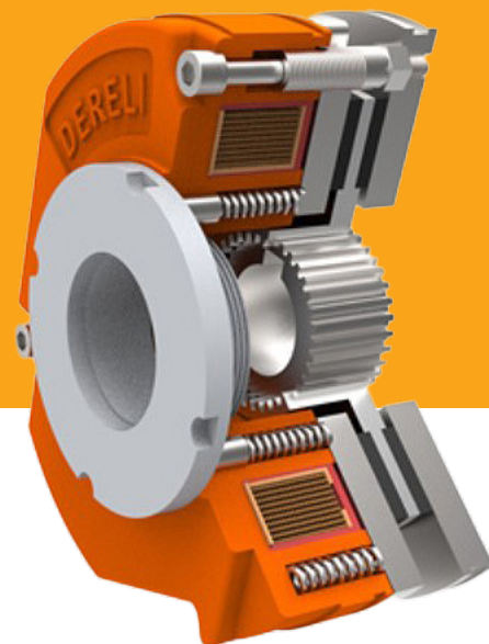
Electromagnetic Brake
